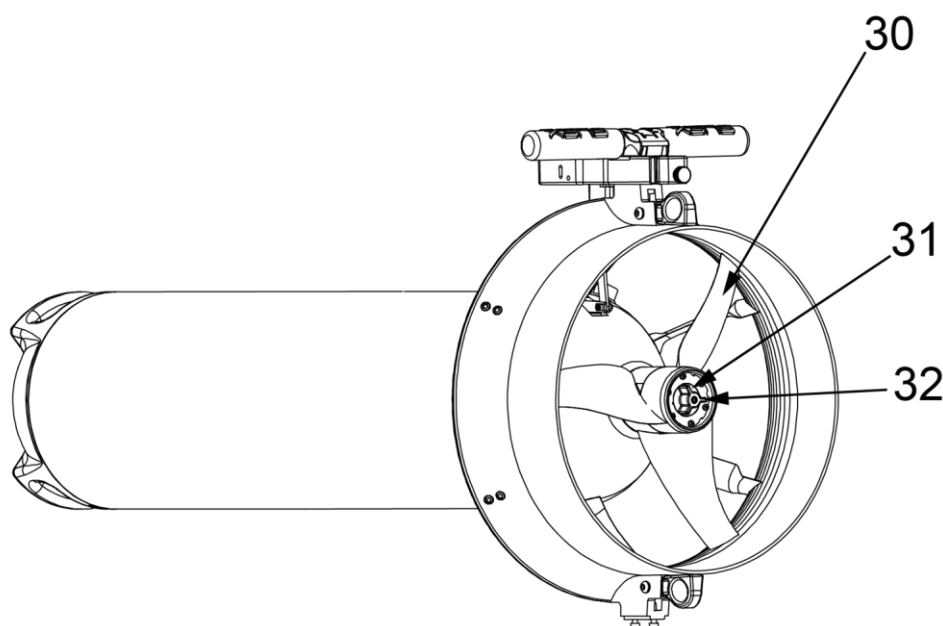
Fig 34 - Propeller extraction
