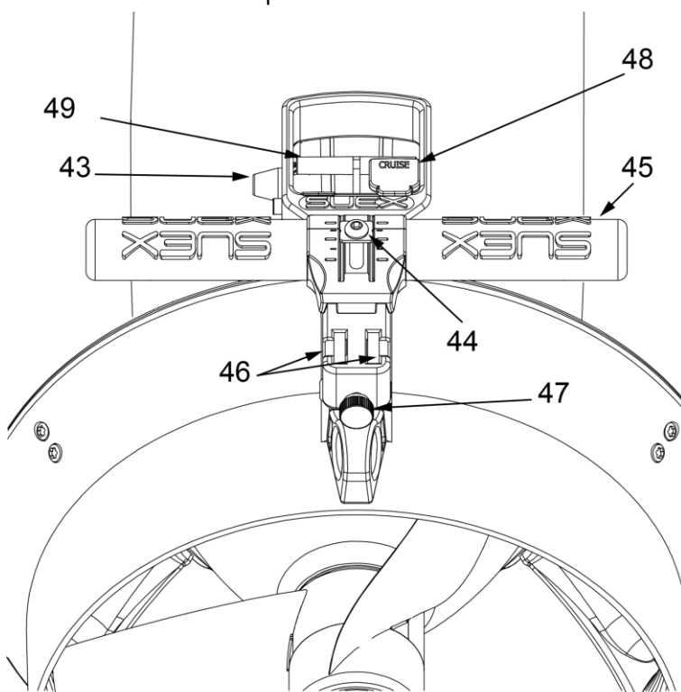
Fig 18 - Controls on handle
