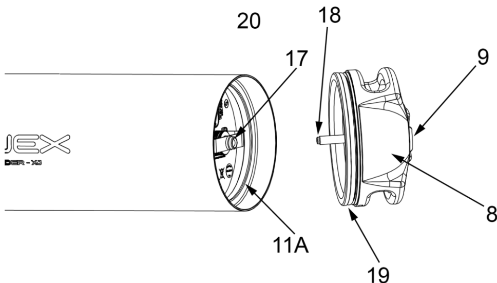
Fig 33 - Closing battery compartment
