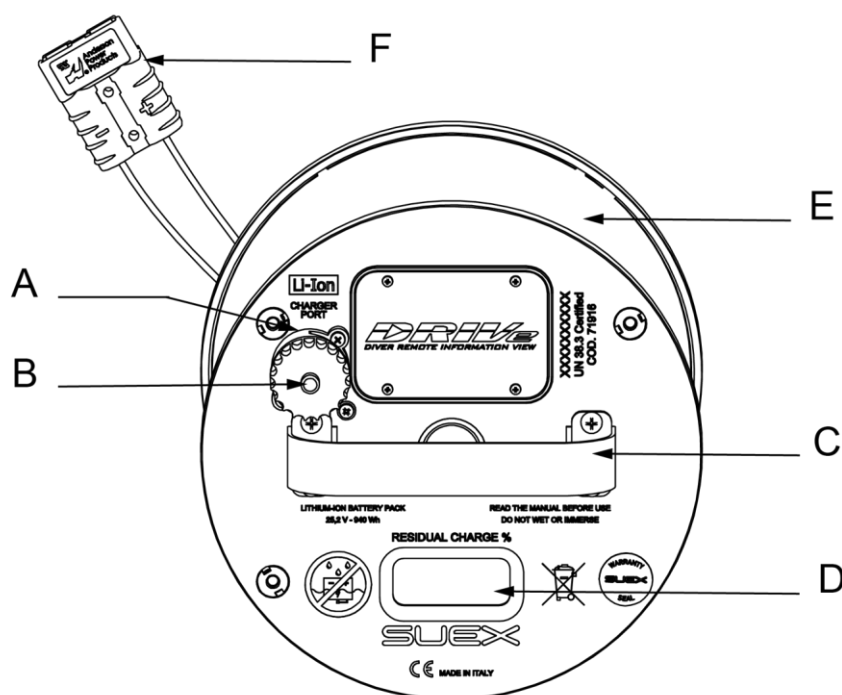
Fig 29 - Battery
