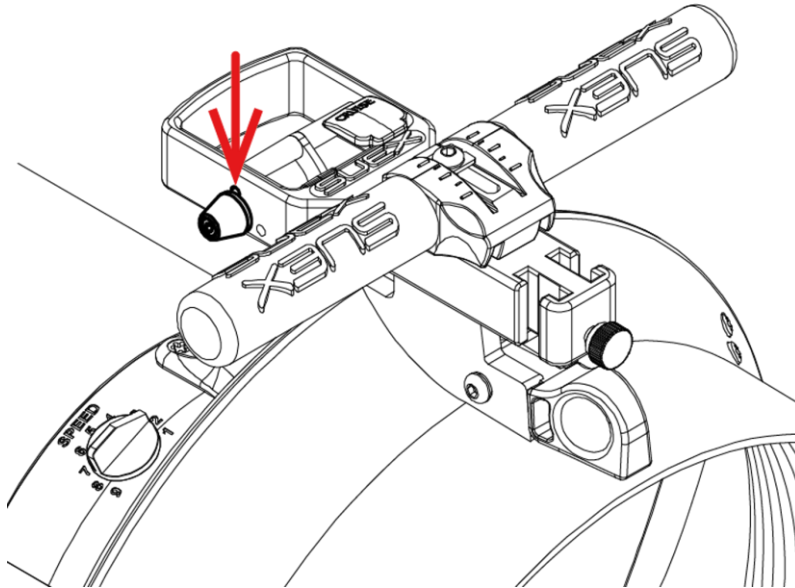
Fig 21 - Turning OFF cruise control
