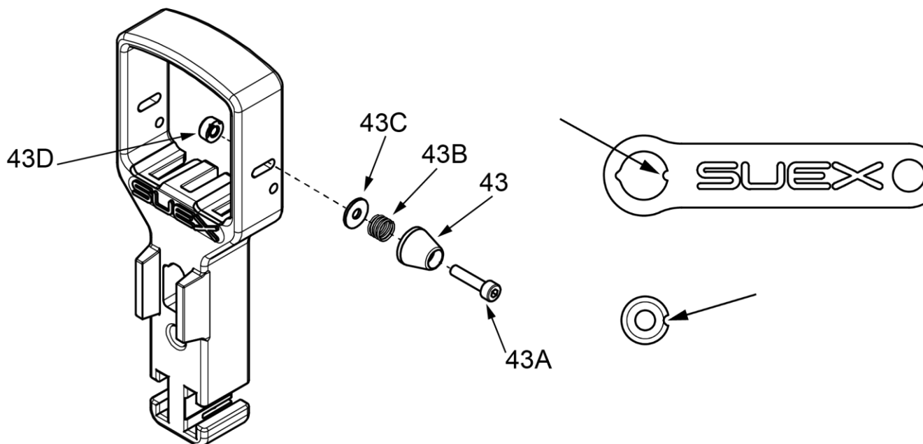
Fig 22 - Place cruise control on the right side
