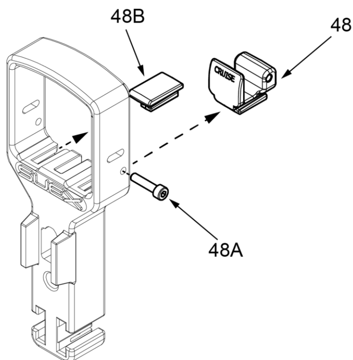
Fig 24 - Place Finger rest on left side
