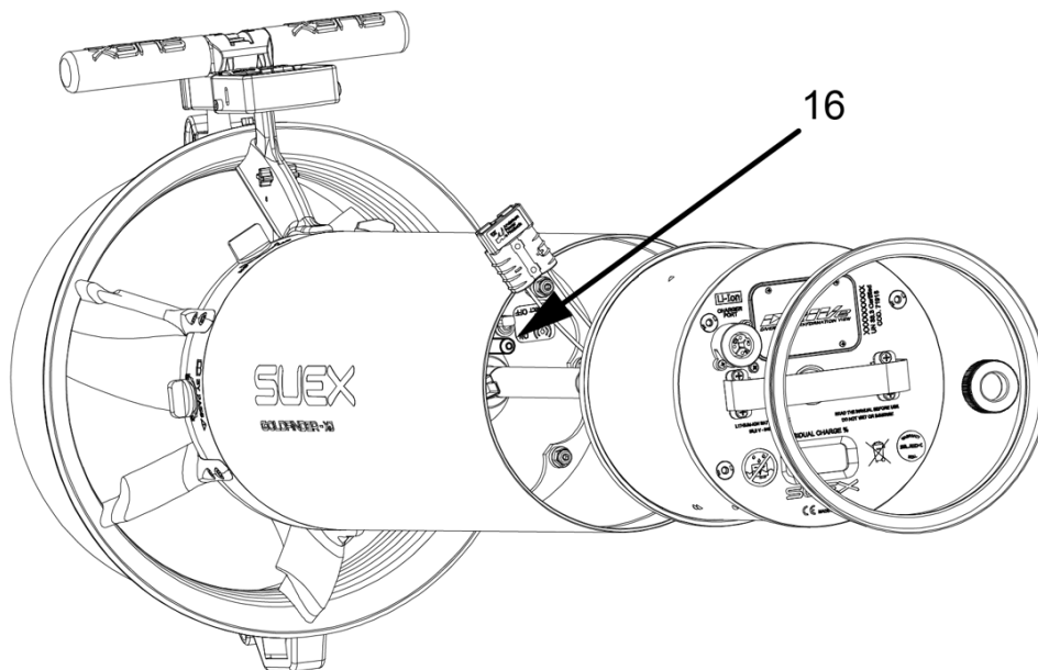
Fig 32 - Antirotation pin
