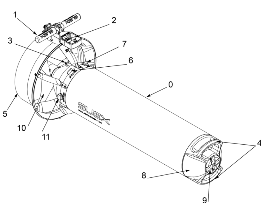
Fig 1 - Part description
