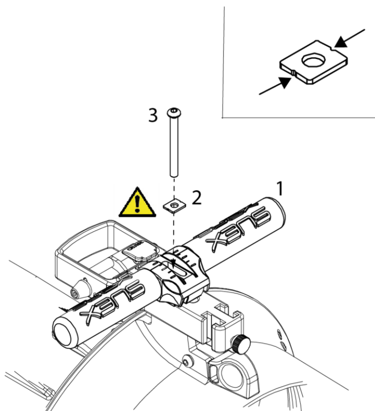
Fig 7 - Handle installation
