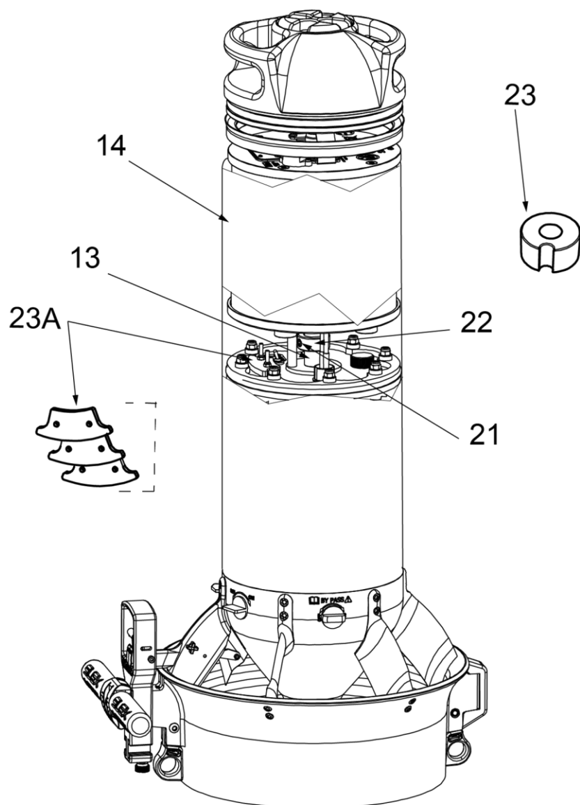
Fig 16 - Ballast placement
