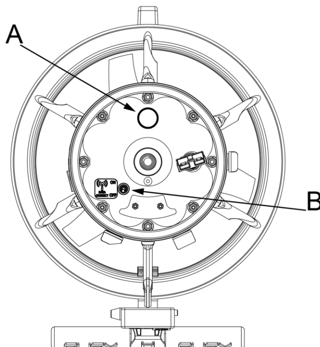
Fig 31 - Vacuum Valve - Antenna Switch
