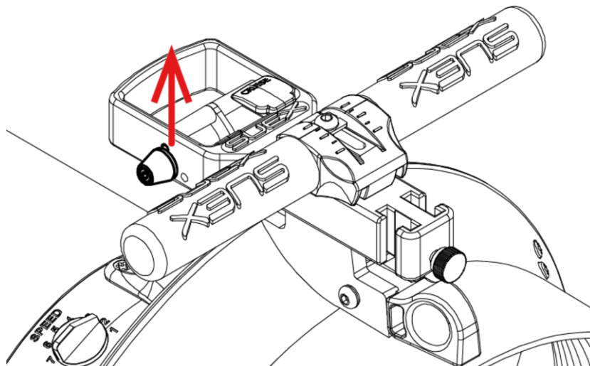
Fig 20 - Cruise control activation
