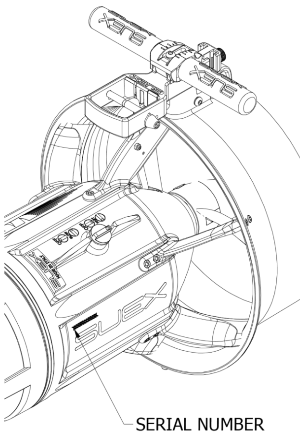
Fig 4 - Serial number
