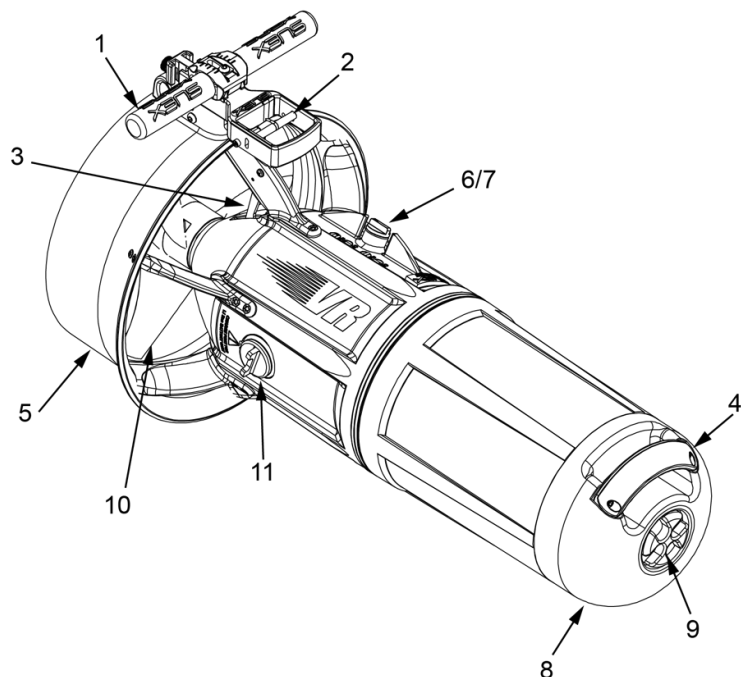
Fig 1 - Part description
