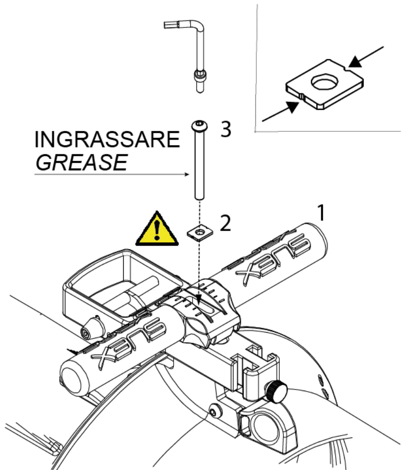
Fig 6 - Handle installation
