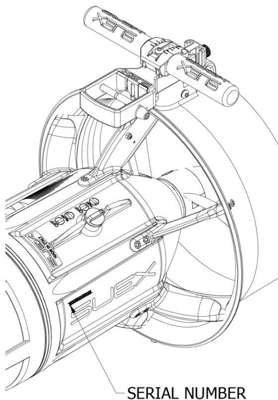
Fig 4 - Serial number
