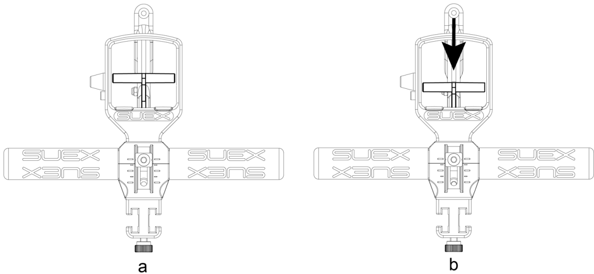
Fig 18 - Trigger position
