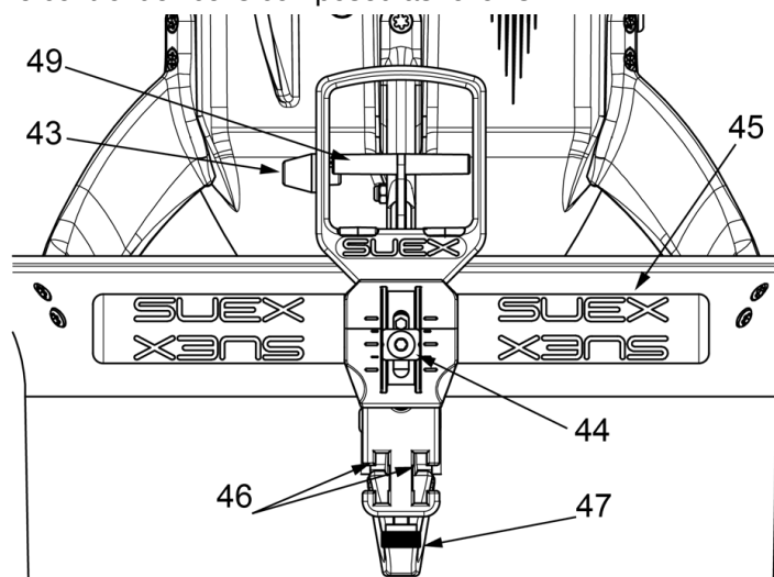
Fig 17 - Controls on handle
