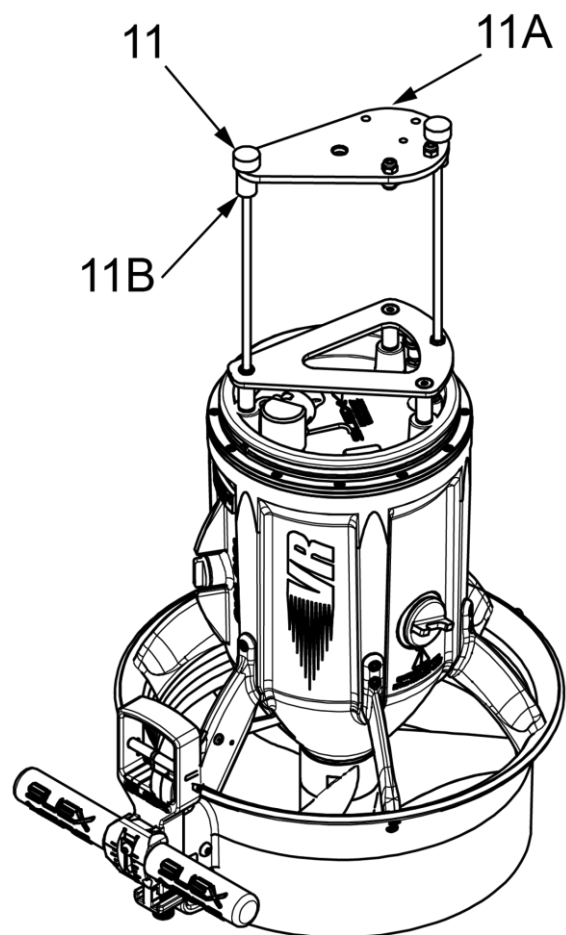
Fig 28 - Plate removal
