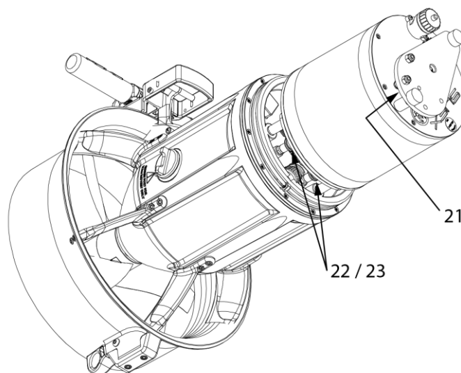
Fig 14 - Ballast insert
