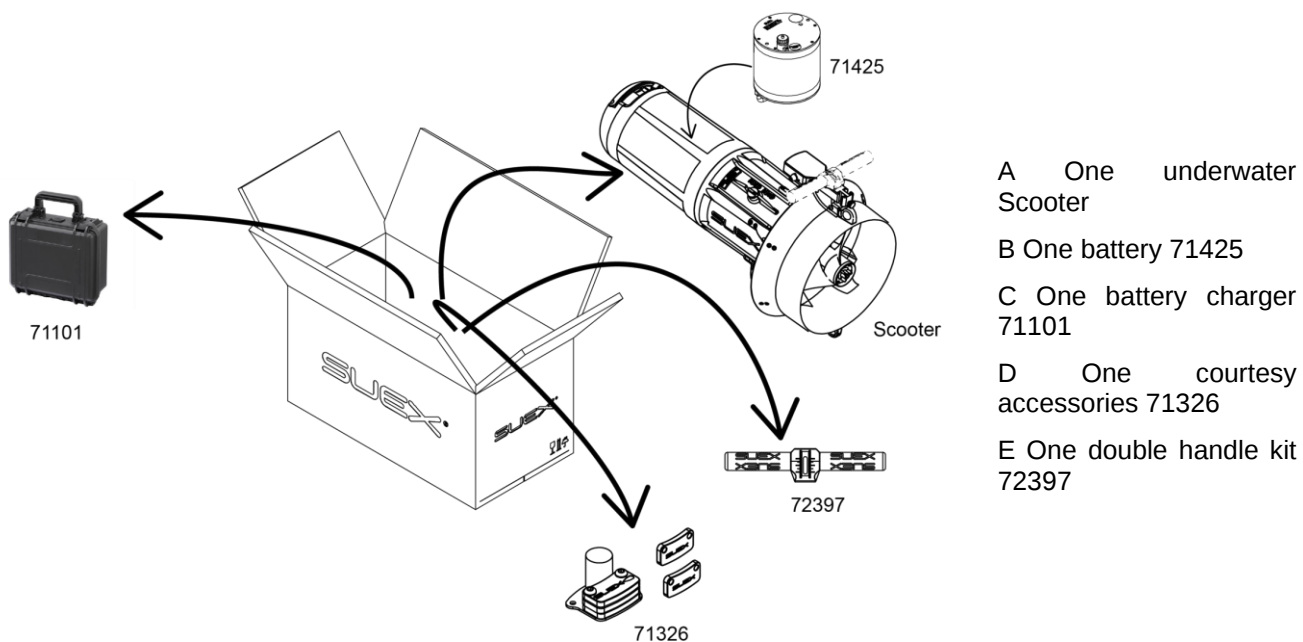
Fig 3 - Package Contents
