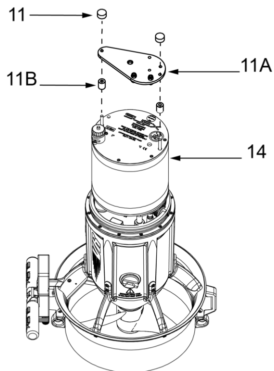
Fig 30 - Battery inserting
