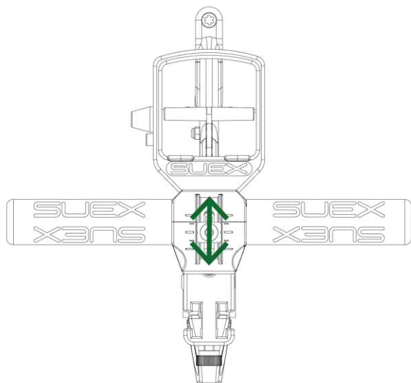
Fig 7 - Adjustment of handle position
