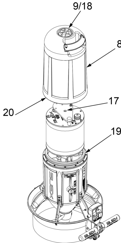
Fig 31 - Closing the battery compartment
