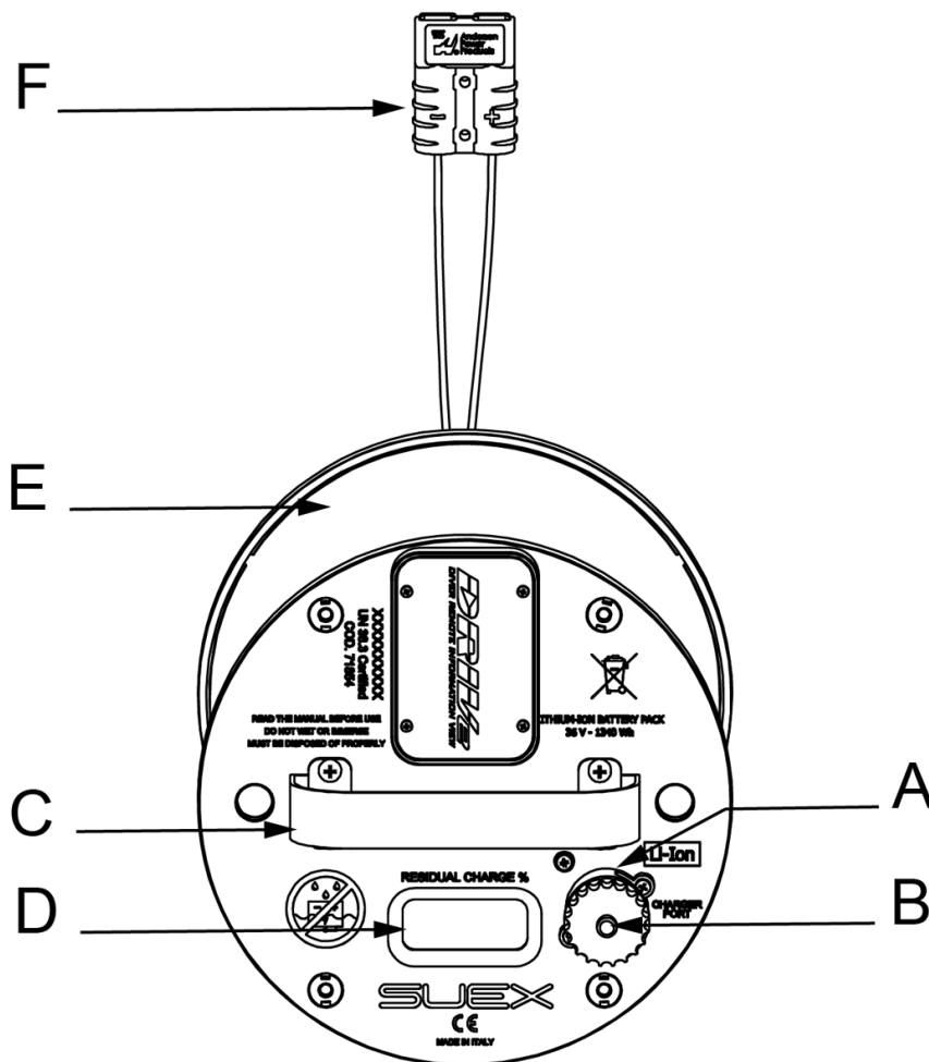
Fig 1 - Parts description
