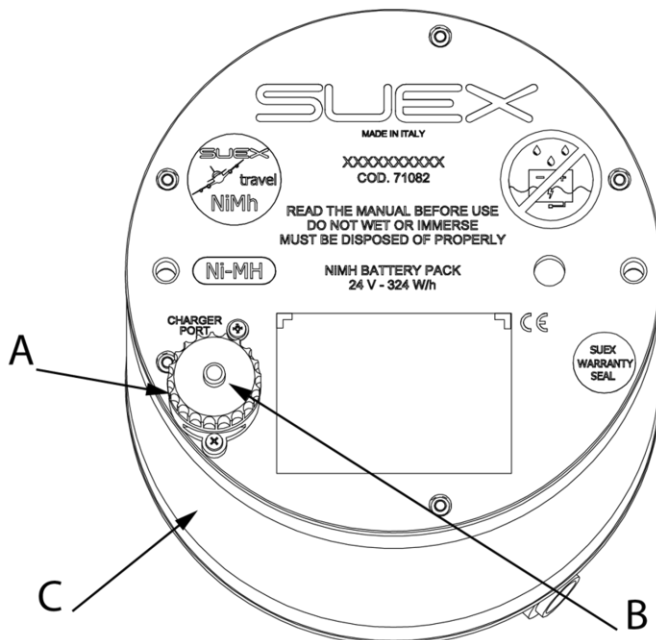
Fig 1 - Battery description
