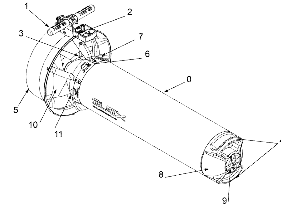
Fig 1 - Part description
