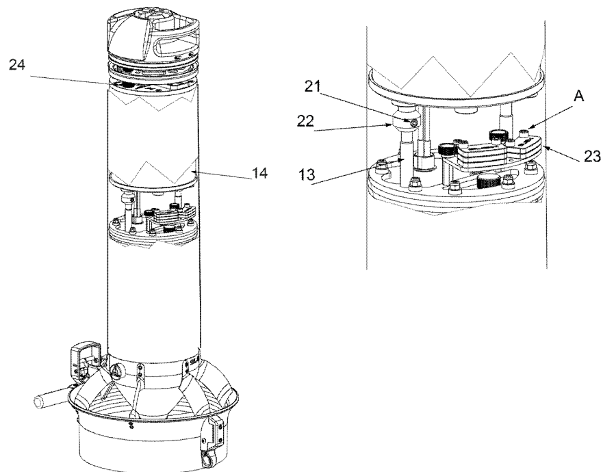
Fig 17 - Ballast placement
