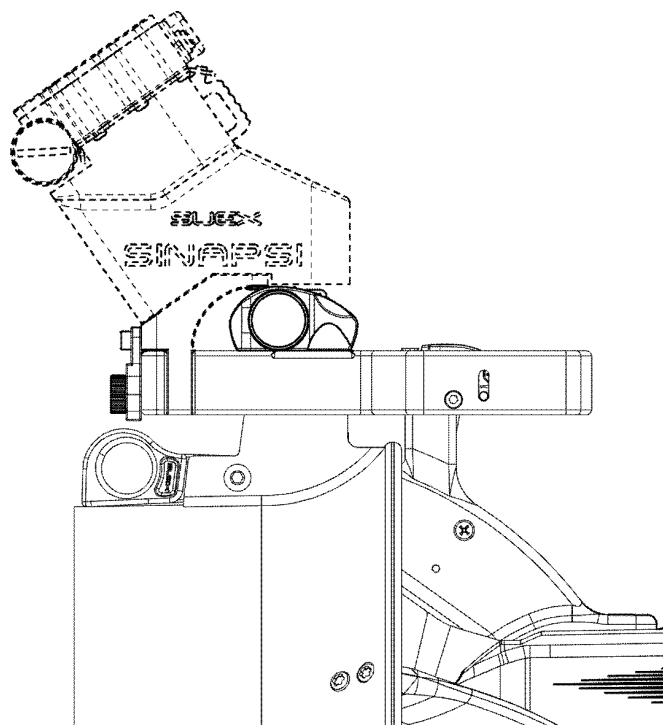
Fig 11 - In case of mounting support
