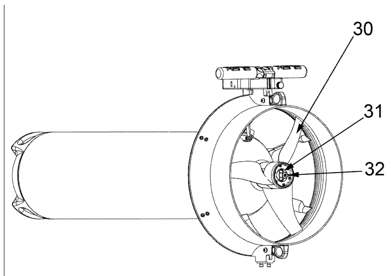
Fig 37 - Propeller extraction
