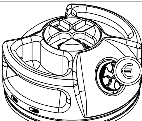
Fig 31 - Use of coin for opening
