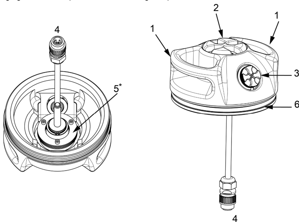
Fig 3 - External charging nose part description
