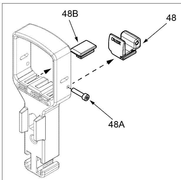
Fig 25 - Place Finger rest on left side
