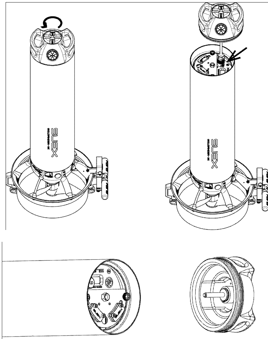
Fig 28 - Battery compartment opening
