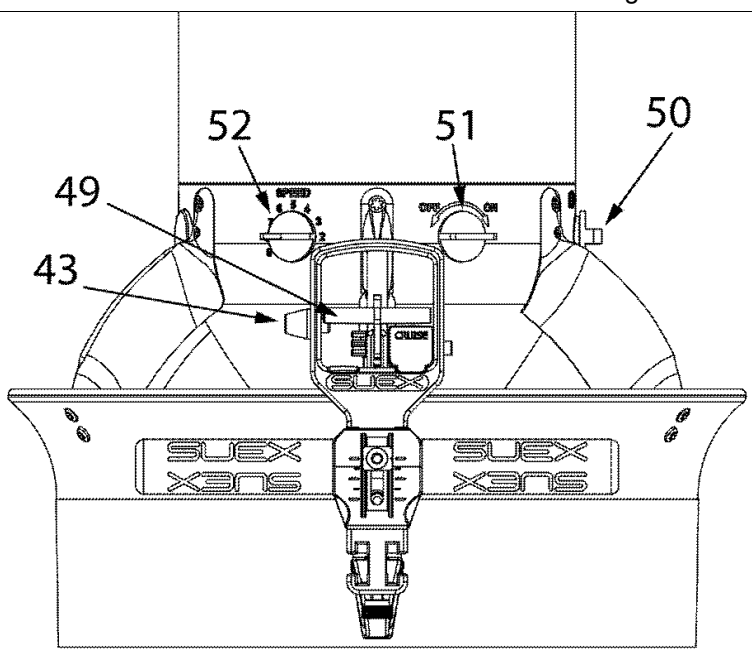
Fig 18 - Scooter Controls
