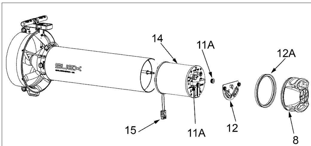
Fig 29 - Battery extraction
