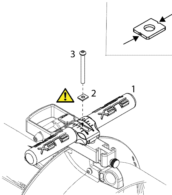
Fig 8 - Handle installation
