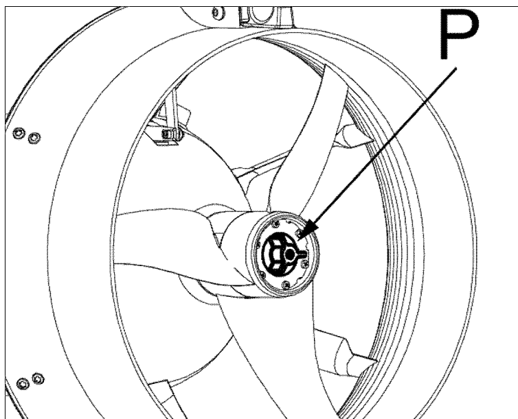
Fig 39 - Turn white knob without forcing
