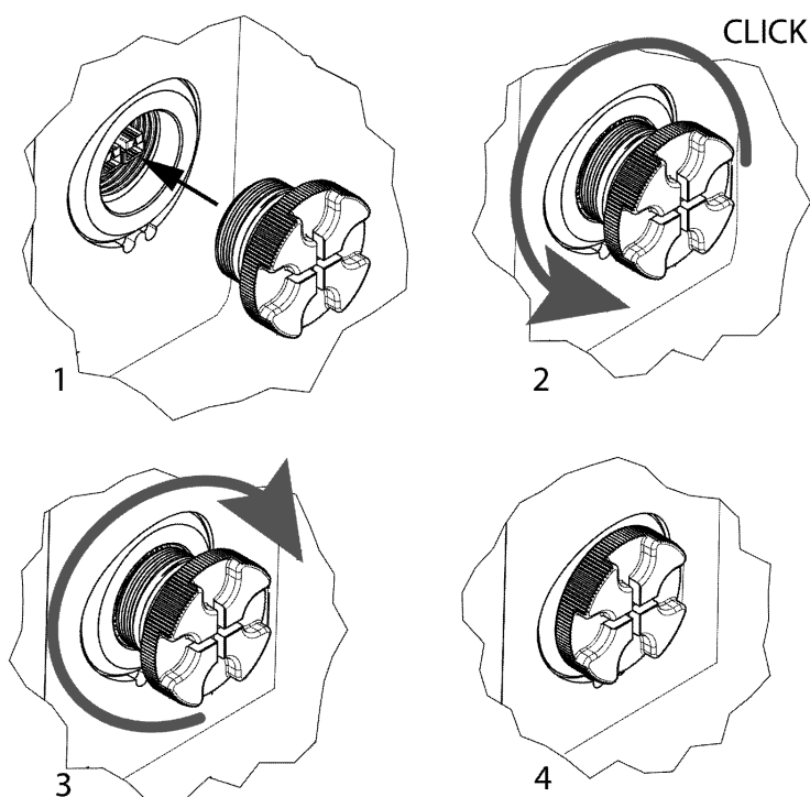
Fig 32 - Correct closure procedure
