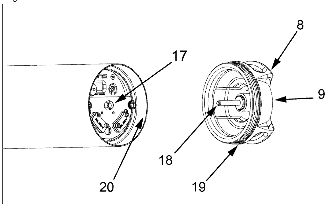
Fig 36 - Closing the battery compartment
