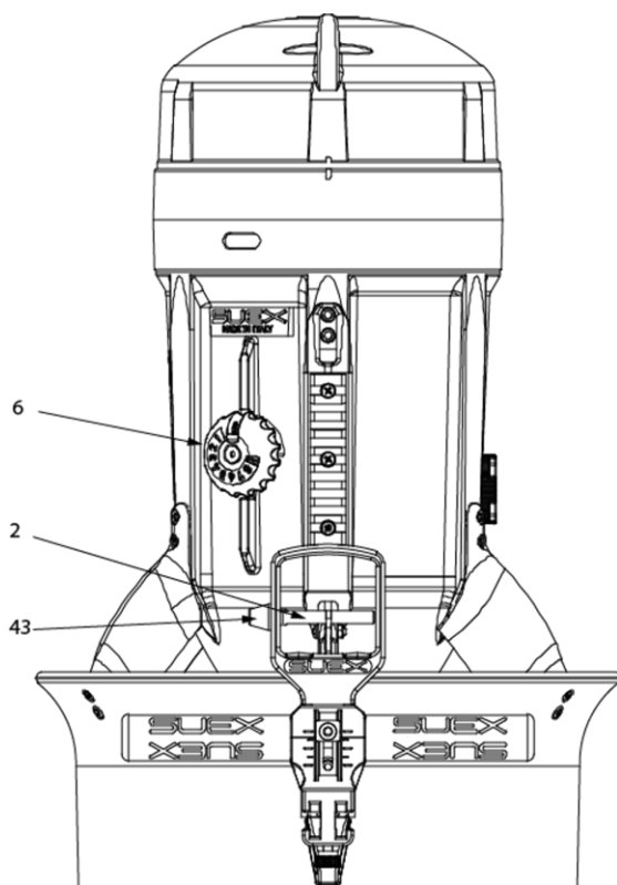
Fig 23 - Scooter controls
