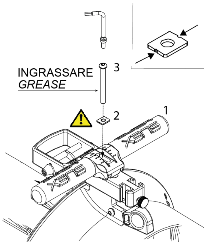
Fig 7 - Handle installation
