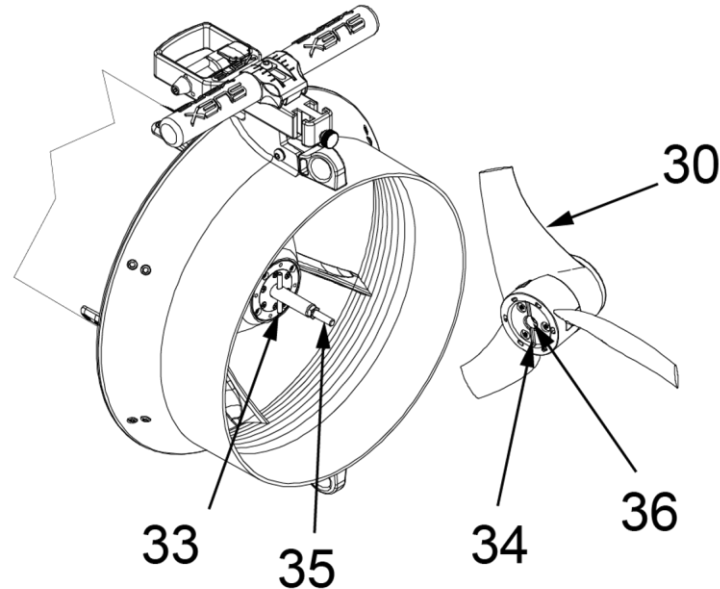
Fig 55 - Propeller insertion
