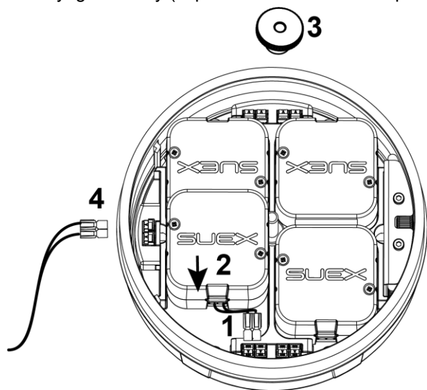
Fig 5 - Voyager battery
