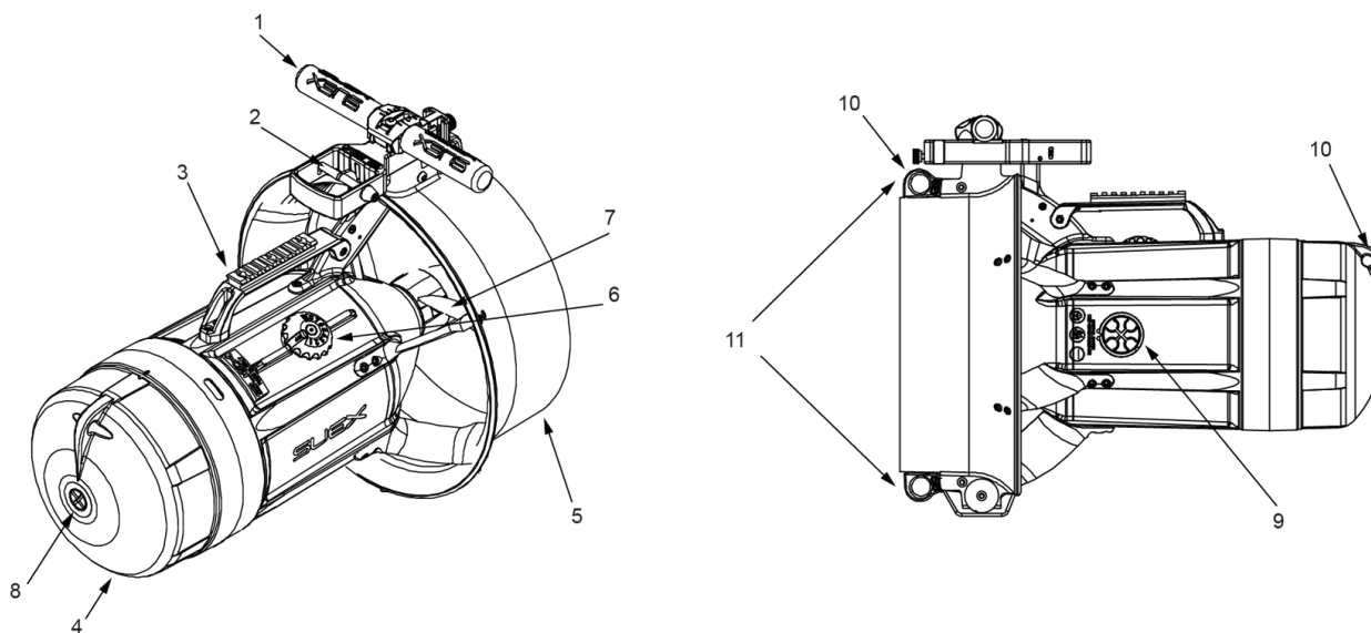
Fig 4 - Parts description
