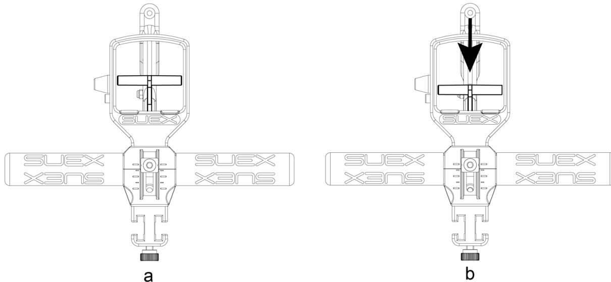
Fig 25 - Trigger position
