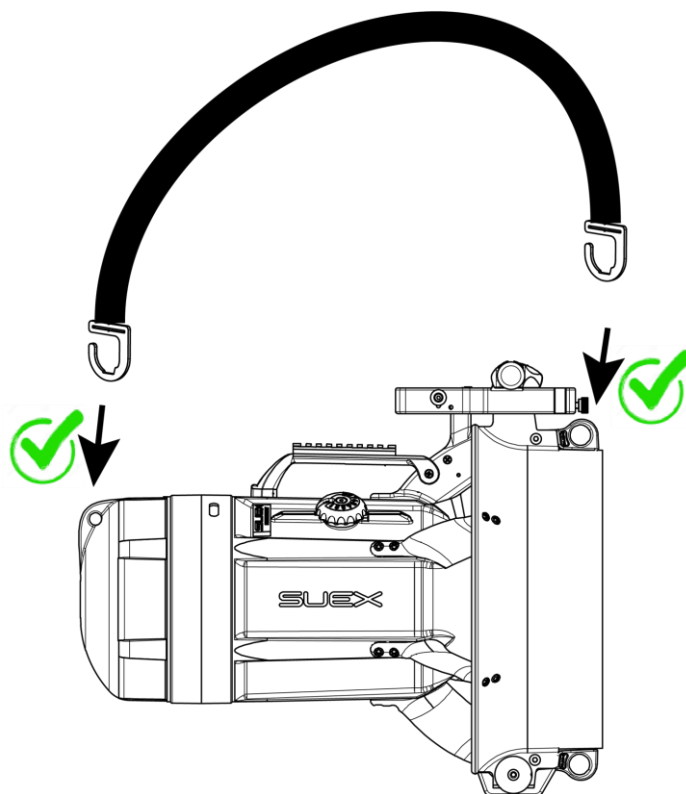
Fig 49 - Stitches for fixing carrying strap
