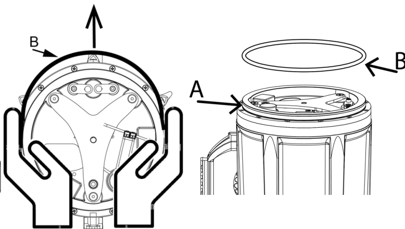
Fig 51 - Apply pressure on the O-ring with both hands simultaneously and push forward
