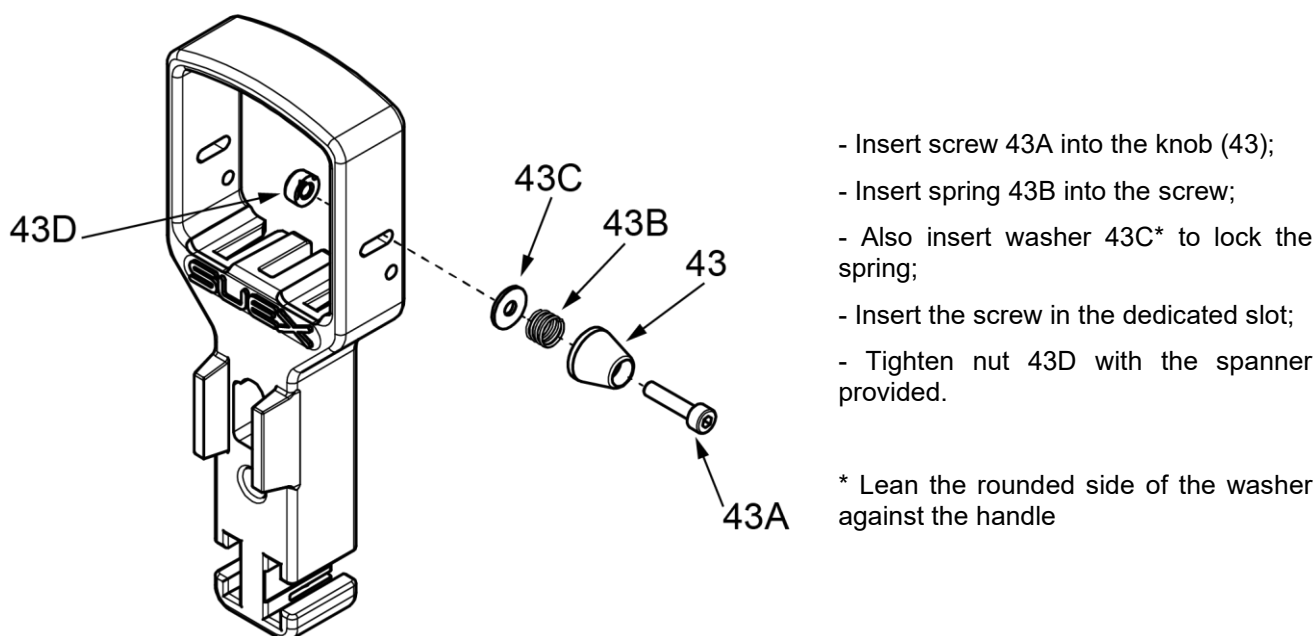
Fig 26 - Cruise control installation
