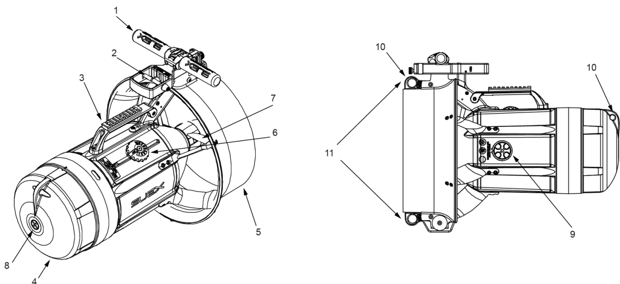
Fig 4 - Parts description
