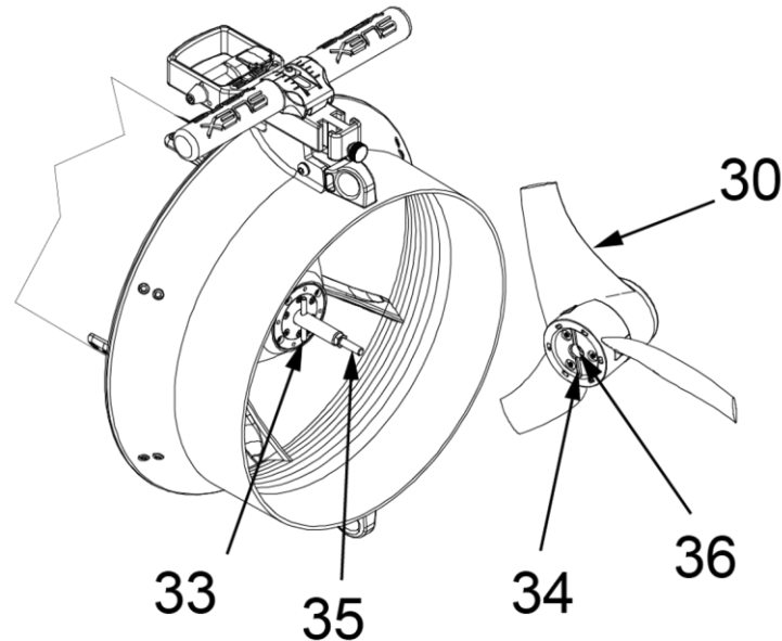
Fig 55 - Propeller insertion
