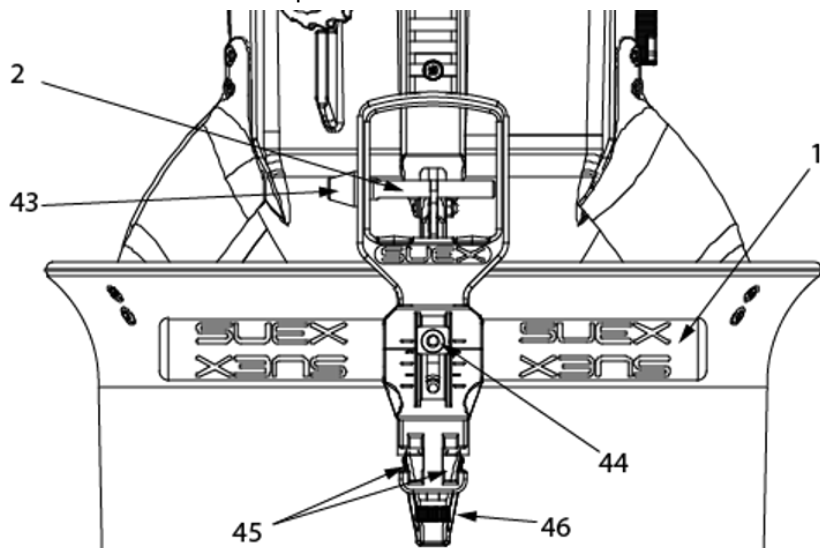
Fig 24 - Controls on handle
