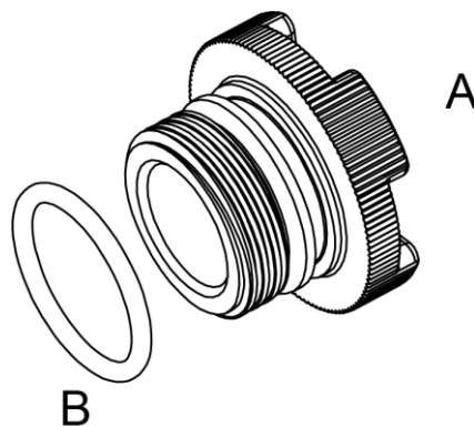
Fig 52 - External charging cap O-ring remove
