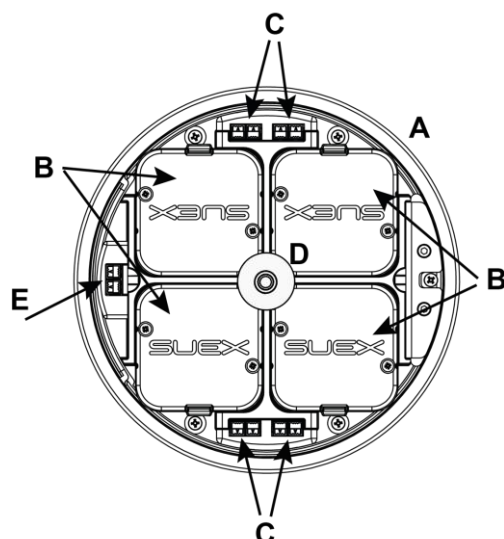
Fig 33 - Voyager battery parts description
