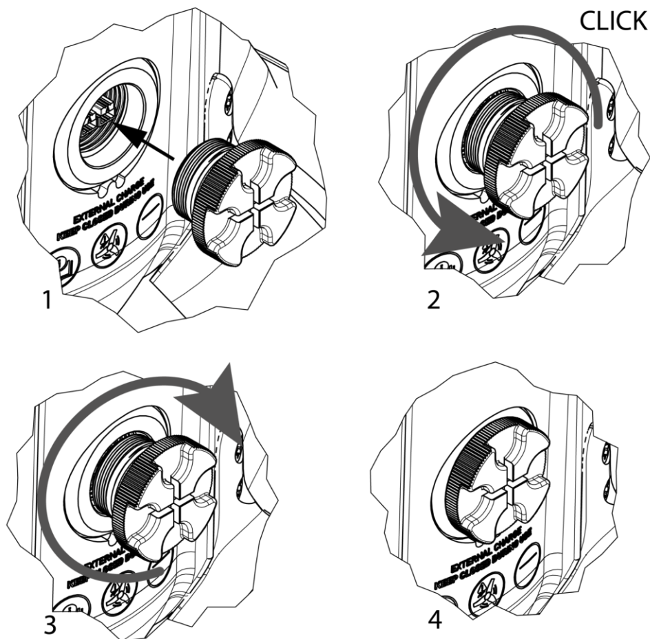
Fig 36 - Correct closure procedure
