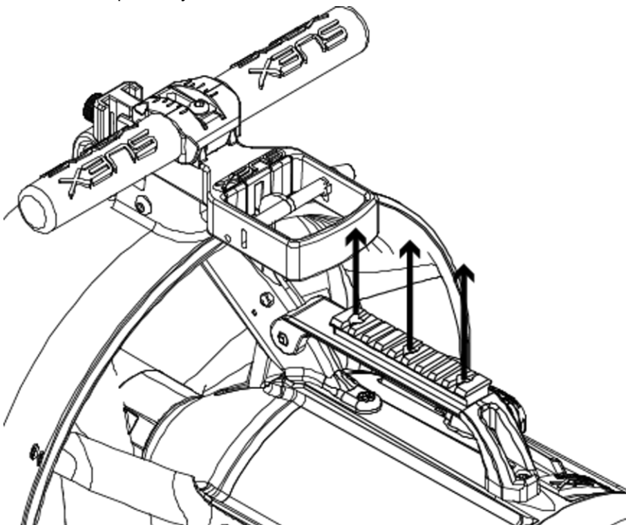
Fig 58 - Picatinny replacement
