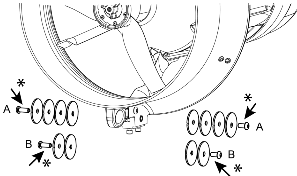
Fig 22 - Outside ballast
