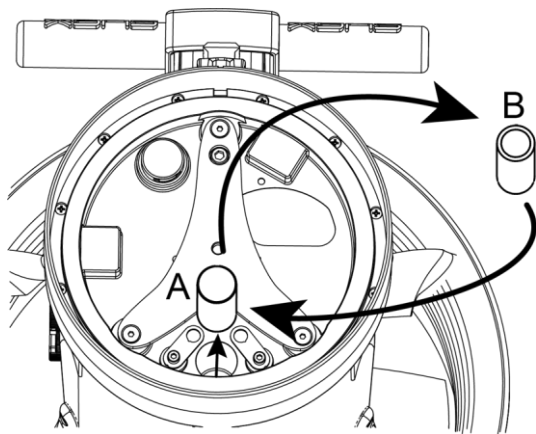
Fig 16 - Ballast replacement
