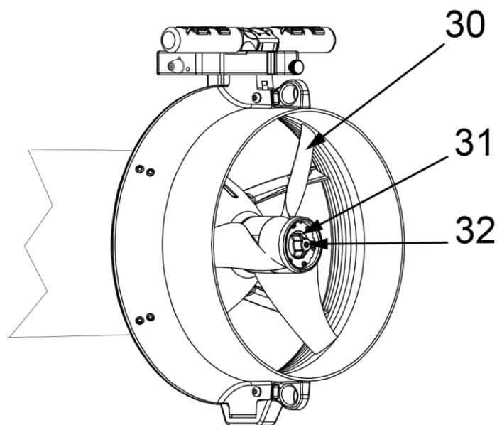
Fig 54 - Propeller extraction
