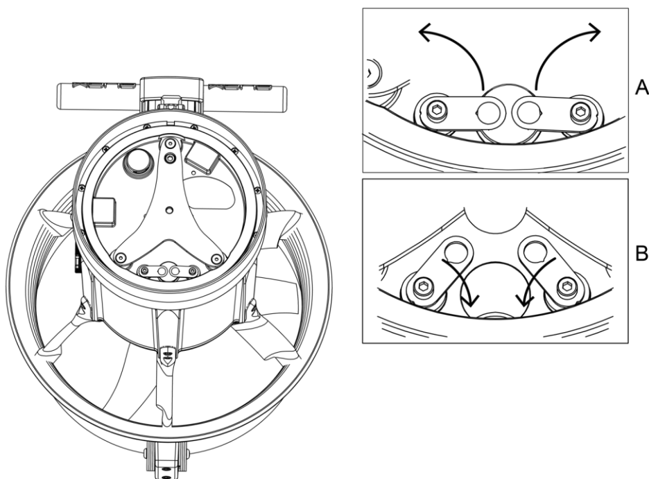
Fig 15 - Opening ballast compartment
