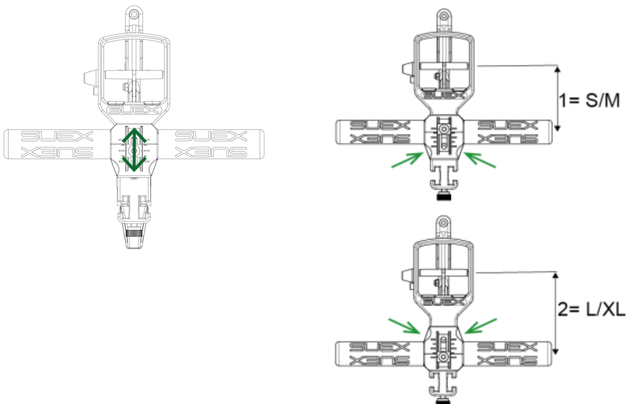
Fig 8 - Adjusting the handle position according to hand size
