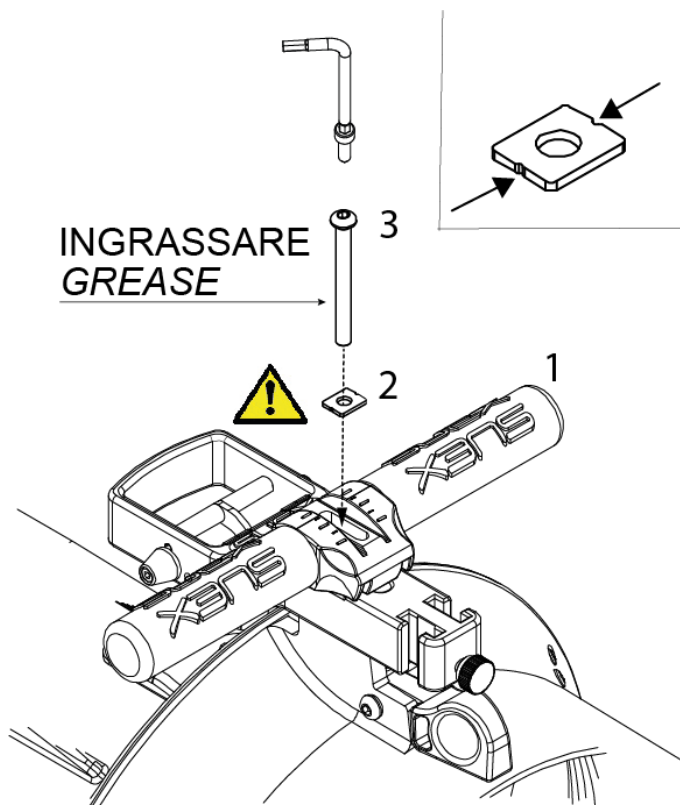
Fig 7 - Handle installation
