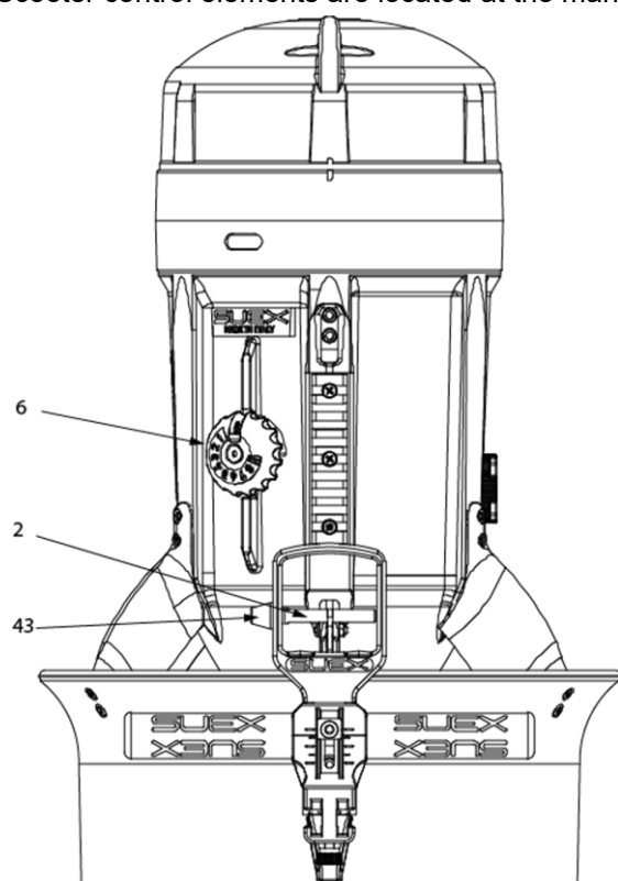
Fig 23 - Scooter controls
