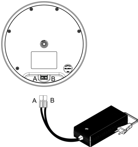
Fig 37 - With Nemo/Quantum battery
