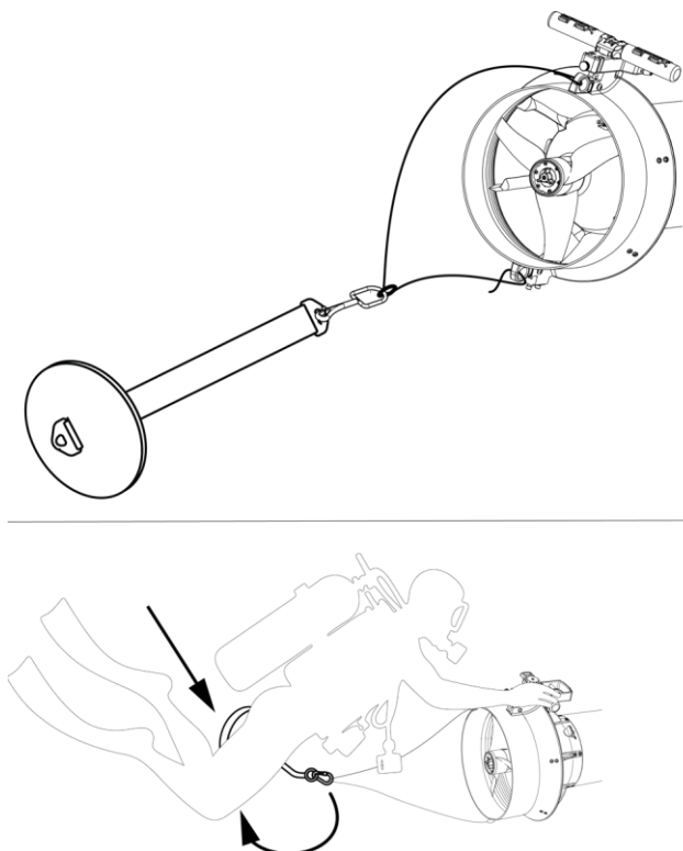
Fig 13 - Dive lift - 72600
